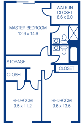
Second Floor / 3 Bedroom
